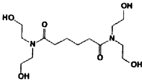
Primid XL-552
