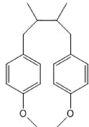
\beta\text{-}\beta'
