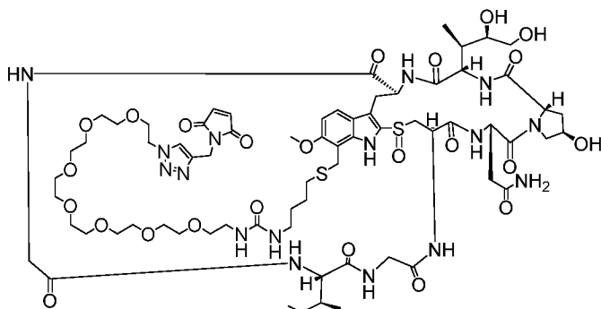
(C6)
